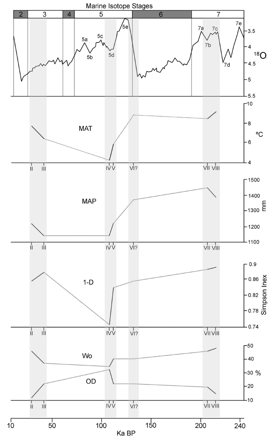
Fig. 27 - San Bernardino cave: representation of mean annual temperature (MAT), mean annual precipitation (MAP), the Simpson small-mammal diversity index (1-D) and the landscape percentages (Wo: woodland + open woodland; OD: open dry + rocky) from the Grotta Maggiore di San Bernardino sequence in relation with the 18O isotope curve (by López-García et al., 2017).
