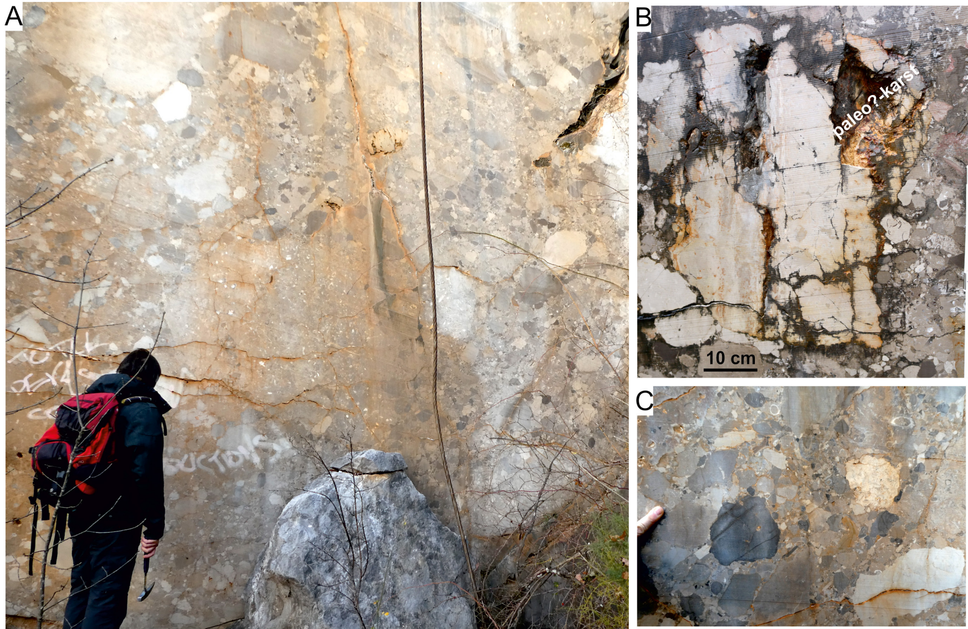
Fig. 18 - Slivia old quarry. A) Mine surface cutting the Slivia breccia. B) Large (paleo?)-karstified block accumulated along with smaller clasts. C) Heterogeneous clasts.
